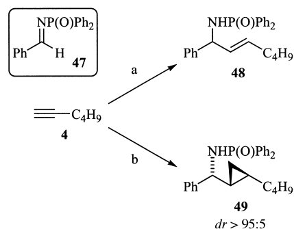
Scheme 8. Solvent dependent formation of allylic amines versus cyclopropyl amines. a) 1. [(Cp) 2 ZrHCl], THF; 2. Me 2 Zn; 3. 47 , 40 °C (65 %); b) 1. [(Cp) 2 ZrHCl], CH 2 Cl 2 ; 2. Me 2 Zn; 3. 47 , reflux (58 %).
