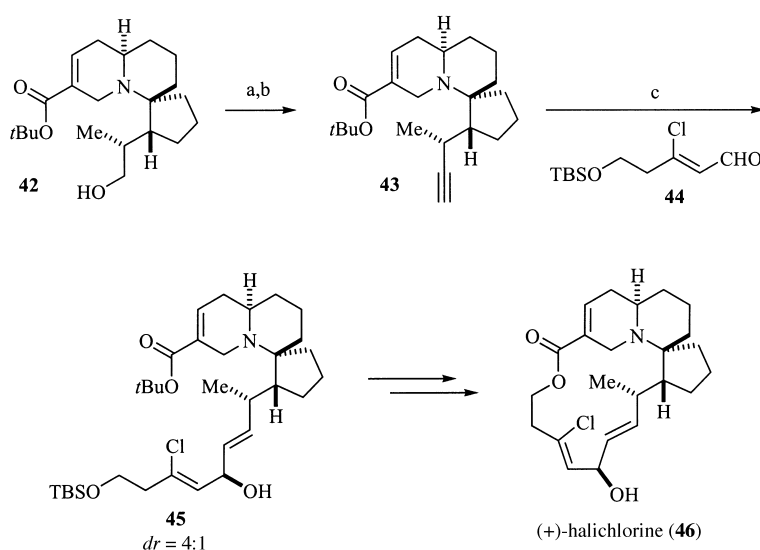
Scheme 7. Asymmetric addition of the alkenyl organometallic derived from alkyne 43 to aldehyde 44 en route to the natural product (+)-halichlorine. a) TPAP, NMO, MeCN; b) N 2 CHP(O)(OMe) 2 , KOtBu, THF (57 % from 42 ); c) 1. [(Cp) 2 ZrHCl], CH 2 Cl 2 ; 2. Me 2 Zn, heptane, 3. 10 mol % ent - 27 ; 4. 44 , –30 °C (67 %).
