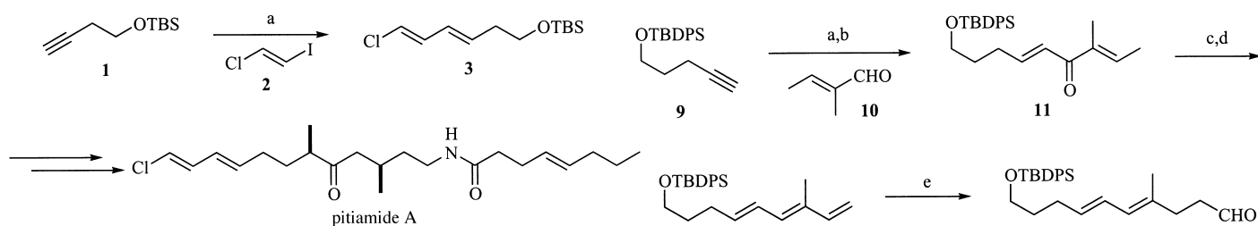
Scheme 1. Use of zirconocene–zinc–palladium triad for the preparation of the chlorodiene segment of the marine natural product pitamide A. a) 1. [(Cp) 2 ZrHCl], THF; 2. ZnCl 2 ; 3. 2 , 8 mol % [Pd(PPh 3 ) 4 ] (85 %).
